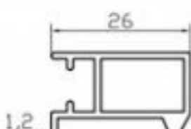
K4417 İÇ RAY PROFİLİ (0.310 Kg/m)
