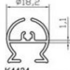
K4424 ARA FİTİLLİ DİKME (0.245 Kg/m)
