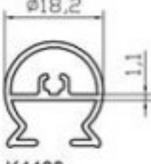
K4400 FİTİLSİZ DİKME (0.215 Kg/m)
