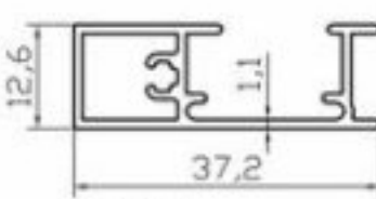
K4407 İÇ RAY PROFİLİ (0.320 Kg/m)
