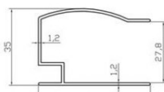
K4426 CAM DİKME PROFİLİ 0.470 Kg/m
