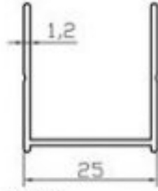
K4412 DUVAR DİKME PROFİLİ (0.240 Kg/m)
