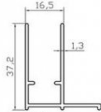
K4409 DUVAR DİKME (0.390 Kg/m)
