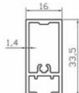
K4406 ASKILIK PROFİLİ (0.430 Kg/m)
