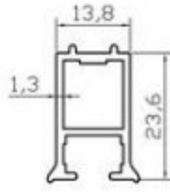
K4405 SABİT DİKME (0.260 Kg/m)
